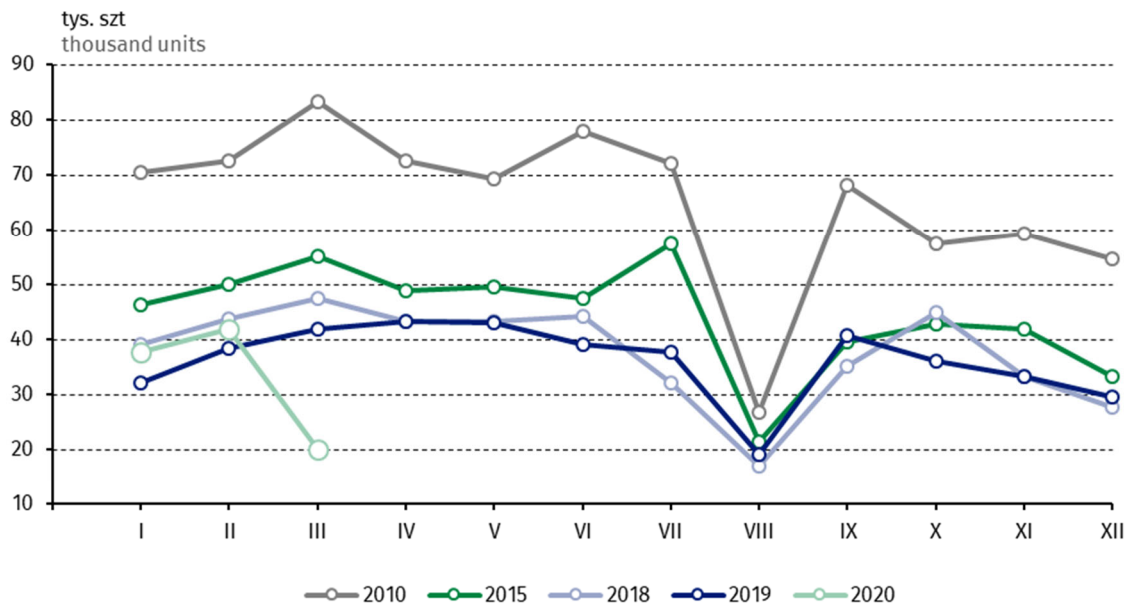
Chart 19. Production of passenger cars a
