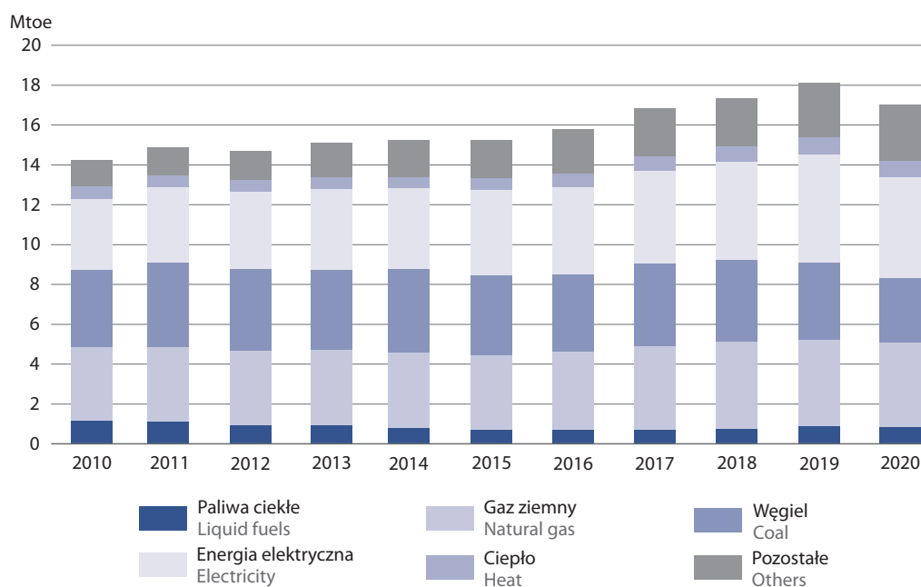
Chart 9. Final energy consumption in industry by carrier
